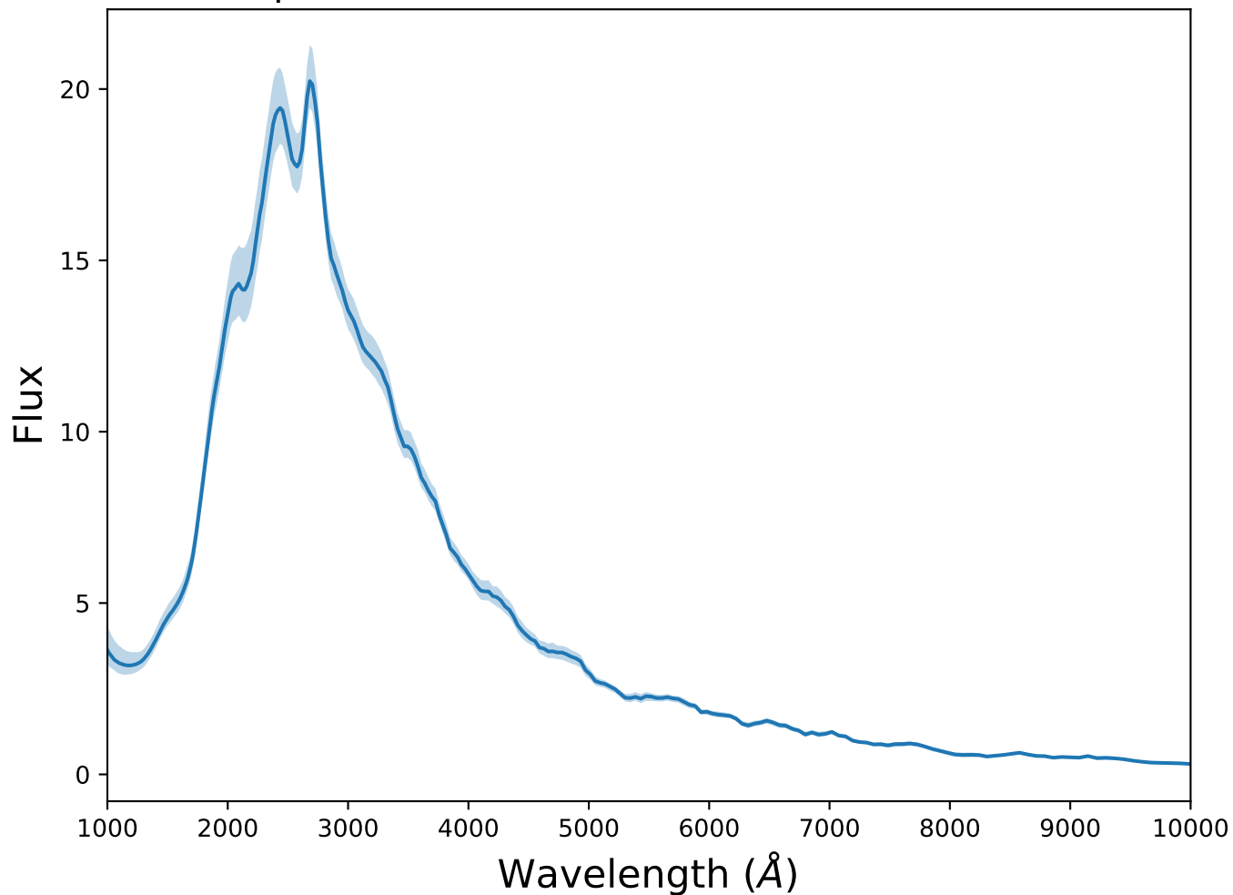
Spectrum 8 for transient CCSN at z=1.09
